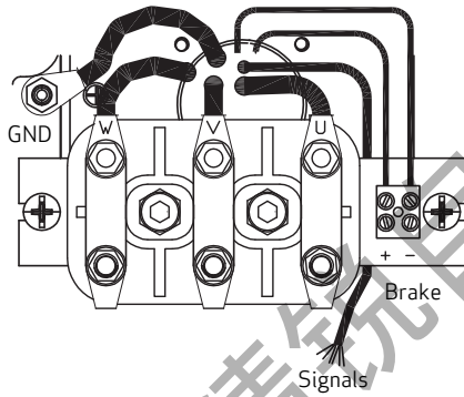
Connection box
